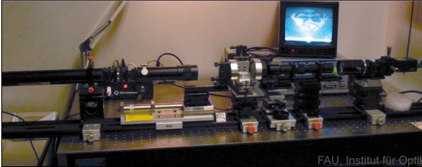
Interferometer for testing micro cylindrical lenses
